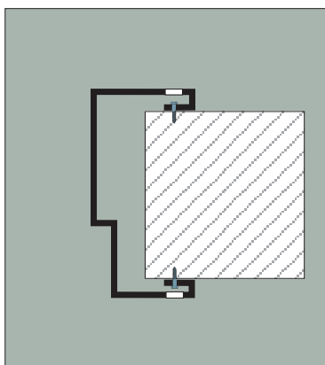
4. R1 rostfri omvik 80 / 100 mm panel
